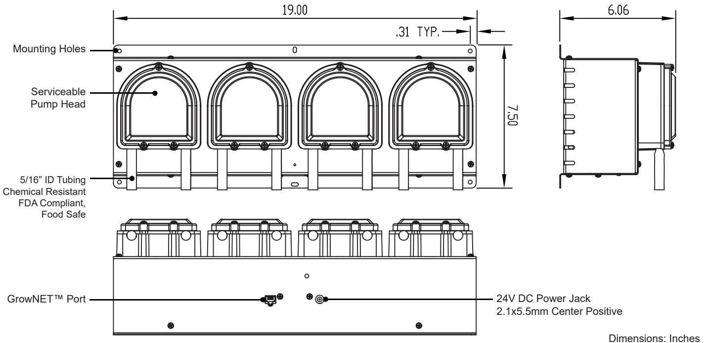
Dimensions: Inches
